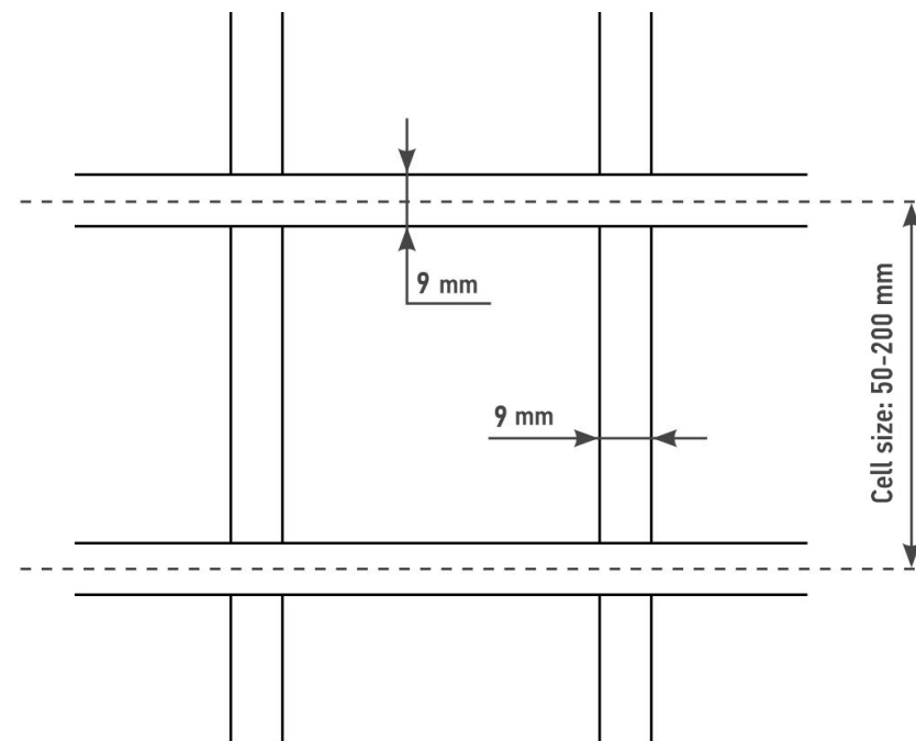
Calculation of components per 1 m 2 of classic open cell ceiling
